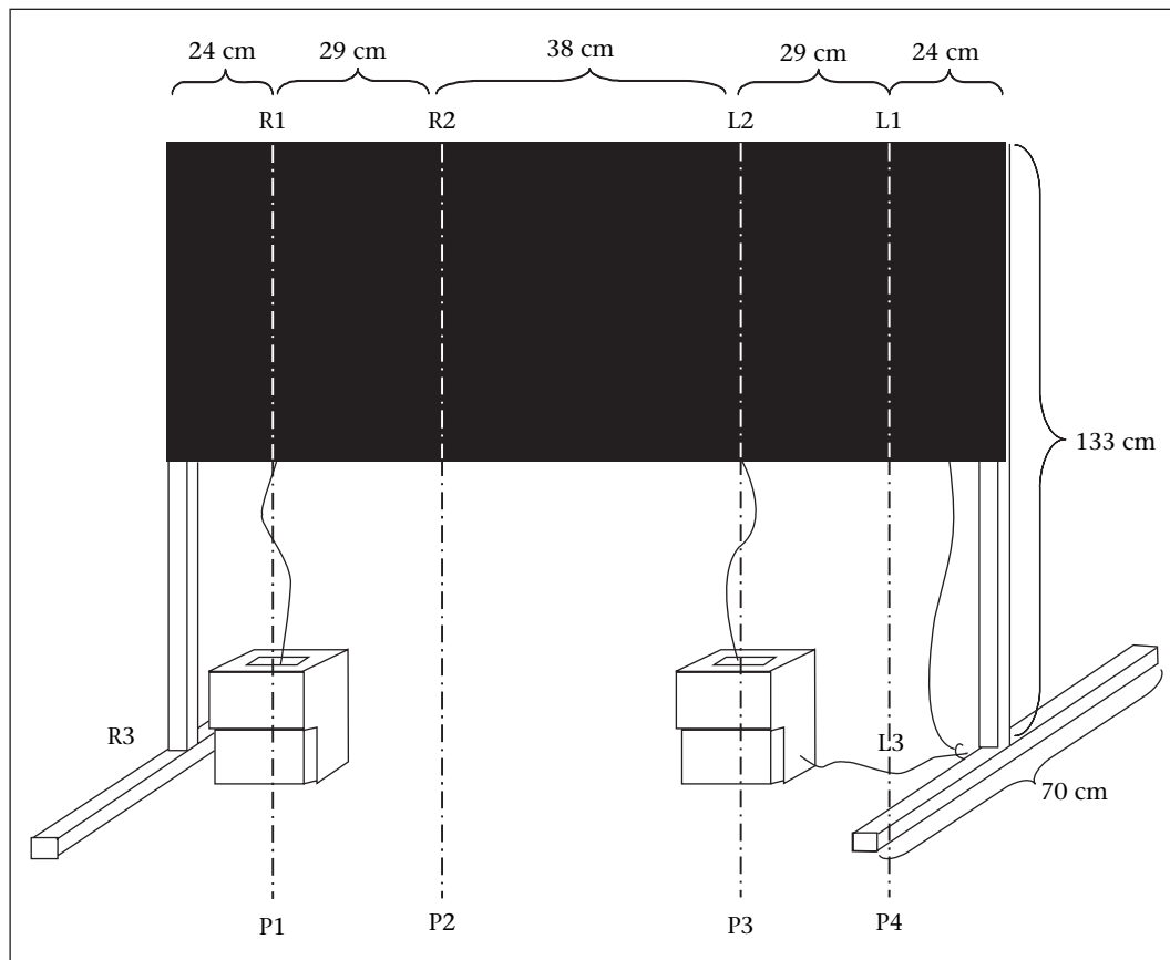
Figure 5. Experimental apparatus. There are six hooks labelled as R1–R3 and L1–L3.
